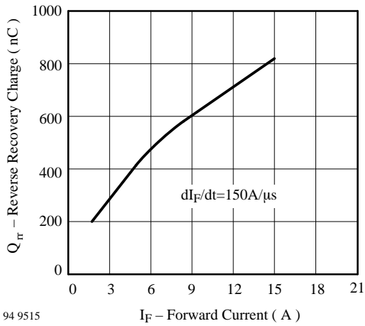
Figure 7 : Reverse Recovery Charge vs. Forward Current
