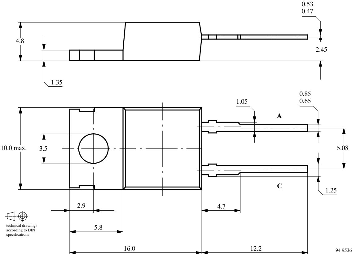
Cathode connected with metallic surface , Plastic Case DO 220 , Weight max.: 2.5 g
